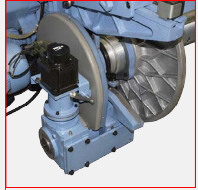
Servo motorlu çözgü salma sistemi Let-off system with servo-motor
